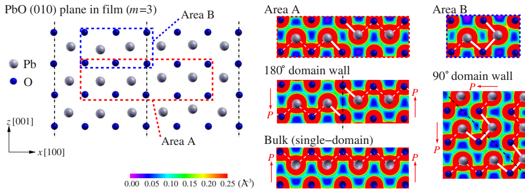
FIG. 5. (Color online) Atomic configuration and charge density distribution on the PbO (010) plane in a PbTiO 3 film three unit-cell thick ( m=3 ) of a Ti-centered domain having a stable period of N_x=6 . Those of the isolated 180° and 90° domain walls and the bulk are shown for comparison. Covalent Pb-O bonds are emphasized by white lines and solid and dashed lines indicate the Pb-O bonds observed near the domain walls and in the bulk, respectively. The dotted-dashed lines indicate the domain walls. Arrows, P , denote the polarization direction in each domain.
